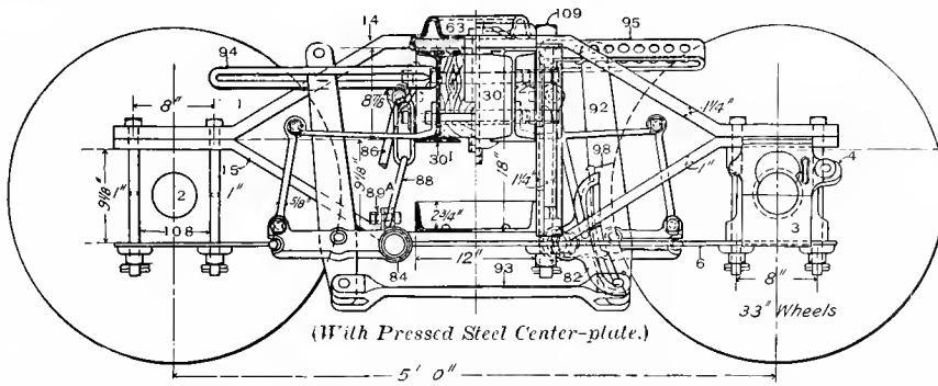
Fig. 4644. Half Longitudinal Section and Half Side Elevation.
